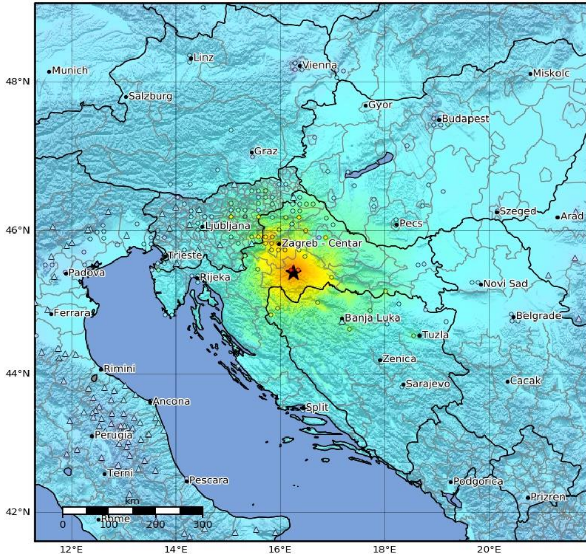
Macroseismic Intensity Map USGS ShakeMap: 3 km WSW of Petrinja, Sisačko-Moslavačka, HR Dec 29, 2020 11:19:54 UTC M6.4 N45.42 E16.26 Depth: 10.0km ID:us6000d3zh
